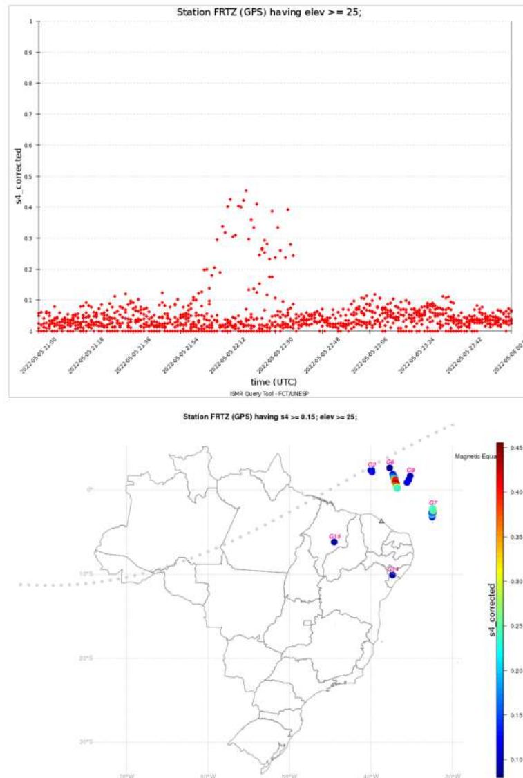
Figure 1: S4 index values corresponding to the GPS constellation for the FRTZ station on 05/05. Between 2100 and 0000 UT (top panel). In the lower panel the map of S4 values > 0.15 for GPS satellites with elevation > 25^\circ in the receiver's field of view from the same station of the upper panel and for the same time interval.
