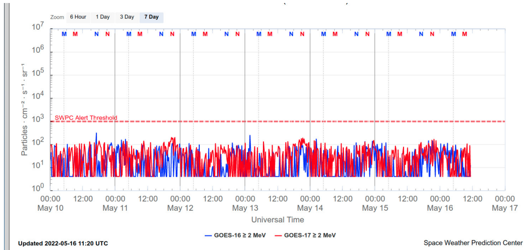
Figure 1: High-energy electron flux ( \geq 2 MeV) obtained from GOES-16 and GOES-17 satellite. Source
