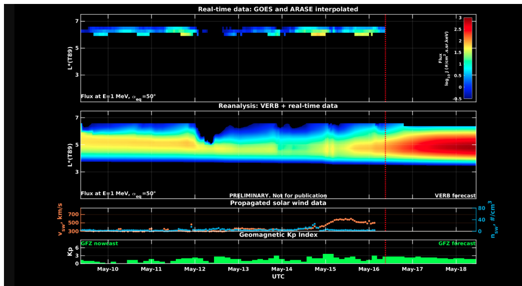
Figure 2: high-energy electron flux data (real-time and interpolated) obtained from ARASE, GOES-16, GOES-17 satellites. Reanalysis's data from VERB code and interpolated electron flux. Solar wind velocity and proton density data from ACE satellite. Source
